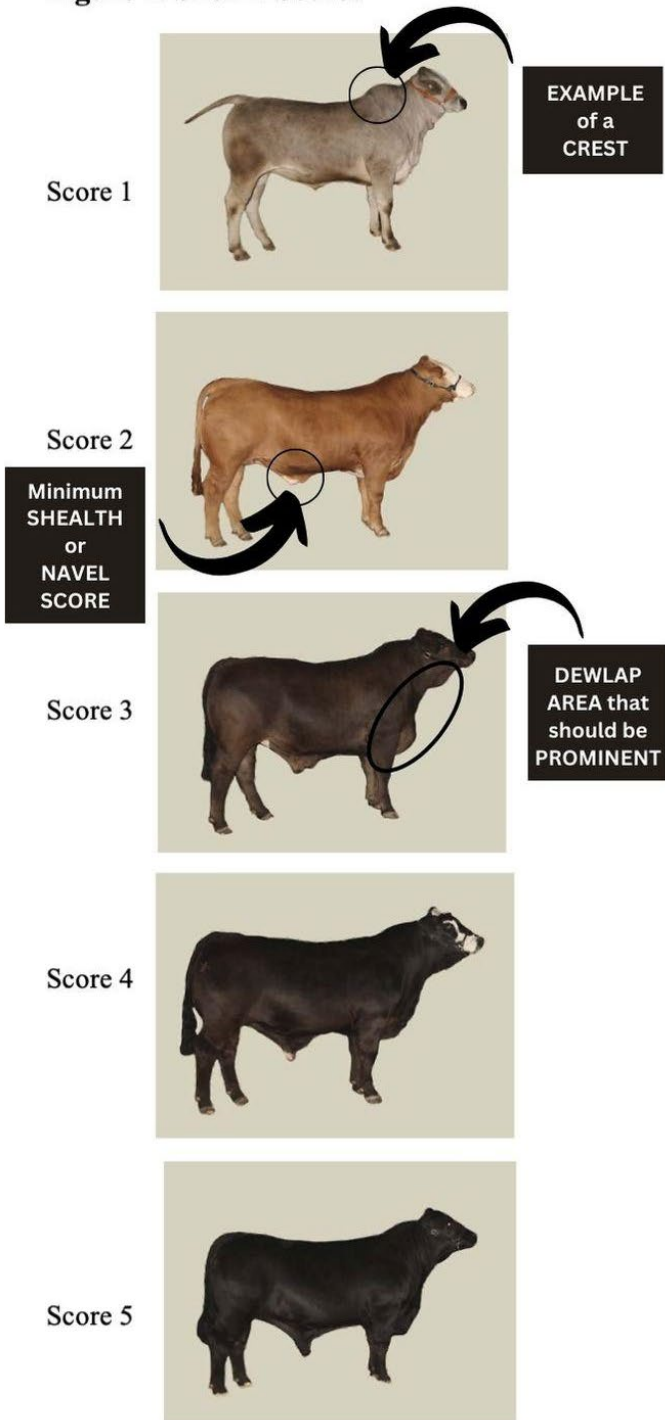
Figure 1. Sheath Scores
