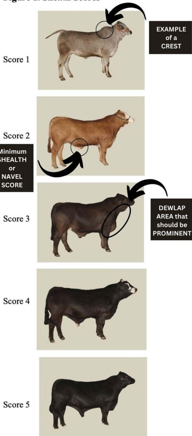
Figure 1. Sheath Scores
